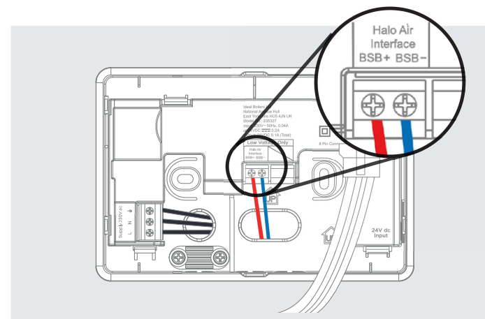
5a. BSB is polarity conscious. Ensure that + and - connections are wired to the same terminal in the heat pump, + to + and - to -.
